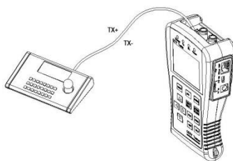
PTZ Controller RS485 Testing
