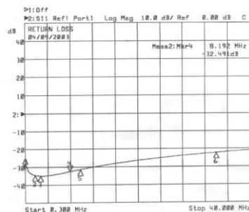
Return Loss
